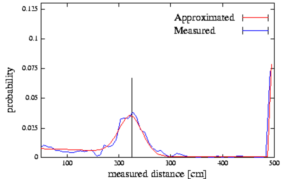
Sonar sensor
